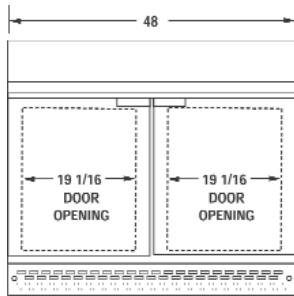
SW48-8C, 10C, 12C-FB FRONT VIEW
