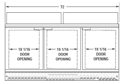
SW72-12C, 18C-FB FRONT VIEW
