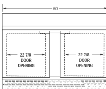
SW60-8C, 12C, 16C-FB FRONT VIEW
