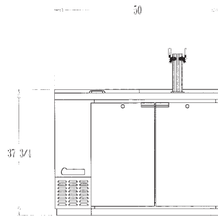
KC50-CT Front View
