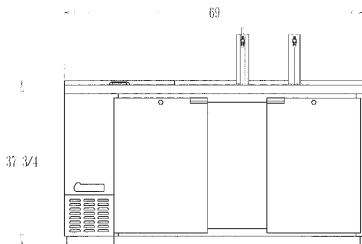
KC69-CT Front View
