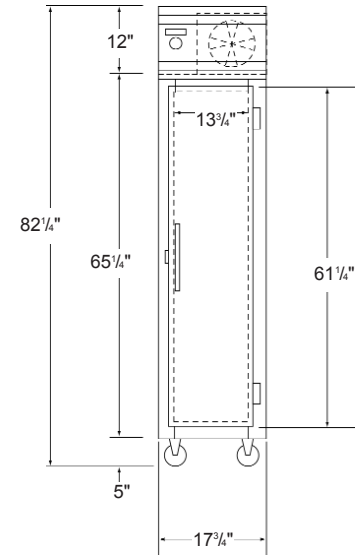
1FSE FRONT VIEW
