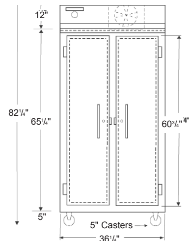
2FSE FRONT VIEW
