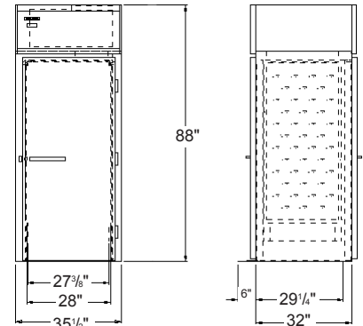
DL1WI-EP FRONT VIEW
