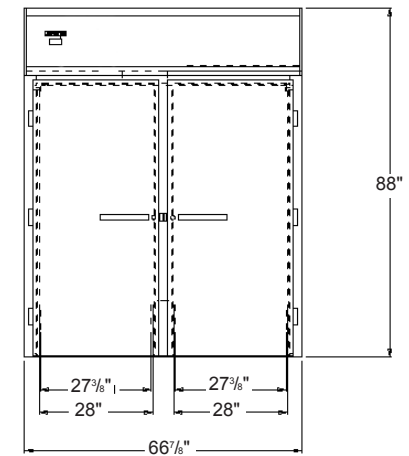
DL2WI-EP FRONT VIEW
