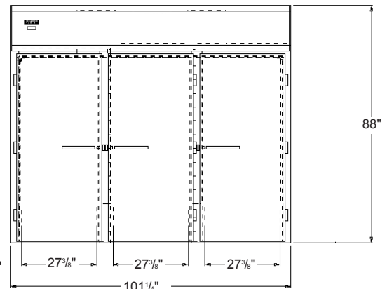
DL3WI-EP FRONT VIEW
