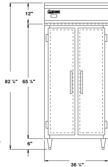
DL2RSE FRONT VIEW
