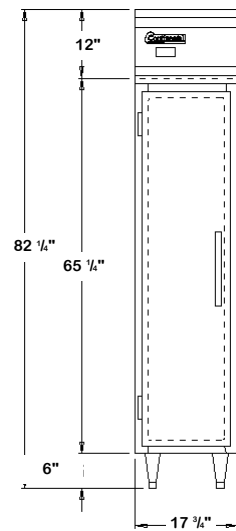
DL1RSE FRONT VIEW
